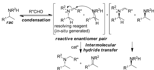
Scheme 1. Approaches for kinetic resolution of racemic amines.
