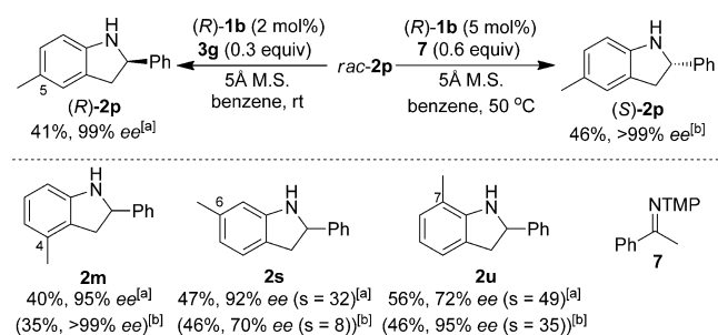
Scheme 3. Enantiodivergent synthesis of 2-substituted indolines. Yields of isolated products reported, ee determined by chiral phase HPLC analysis. [a] Resolutions were carried out on a 0.1 mmol scale with racemic 2 (0.1 mmol), 3g (0.03 mmol), ( R )- 1b (2 mol%), and 5 Å M.S. (50 mg) in benzene (0.1 M) at room temperature for 22 h. [b] Resolutions were carried out on a 0.1 mmol scale with racemic 2 (0.1 mmol), 7 (0.06 mmol), ( R )- 1b (5 mol%), and 5 Å M.S. (50 mg) in benzene (0.1 M) at 50 °C for 19 h.
